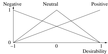
Figure 8: Fuzzy sets for event’s desirability
